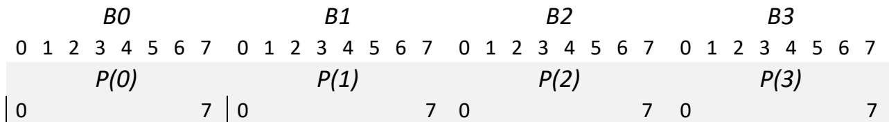
Figure 16 – Packing of 8 bit pixels
