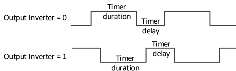
Figure 28 – Output inverters
