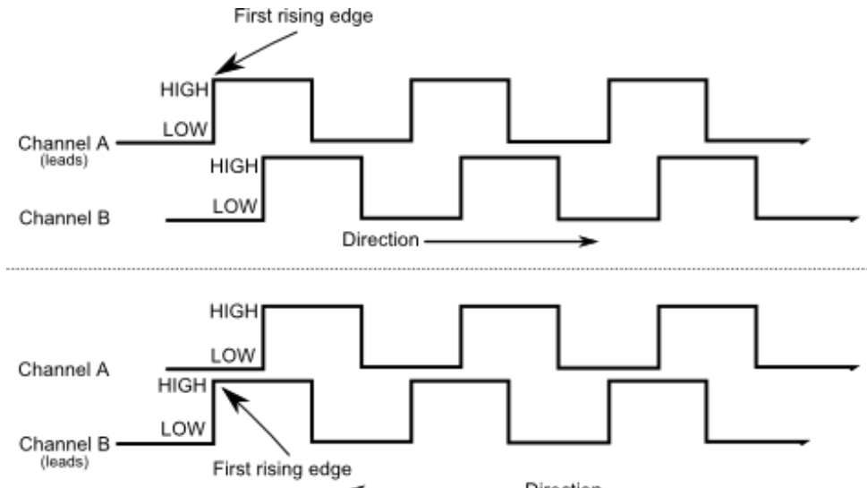
Figure 26 – Encoder channels
