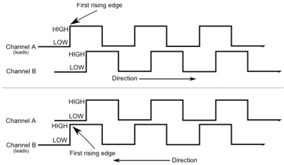
Figure 26 – Encoder channels
