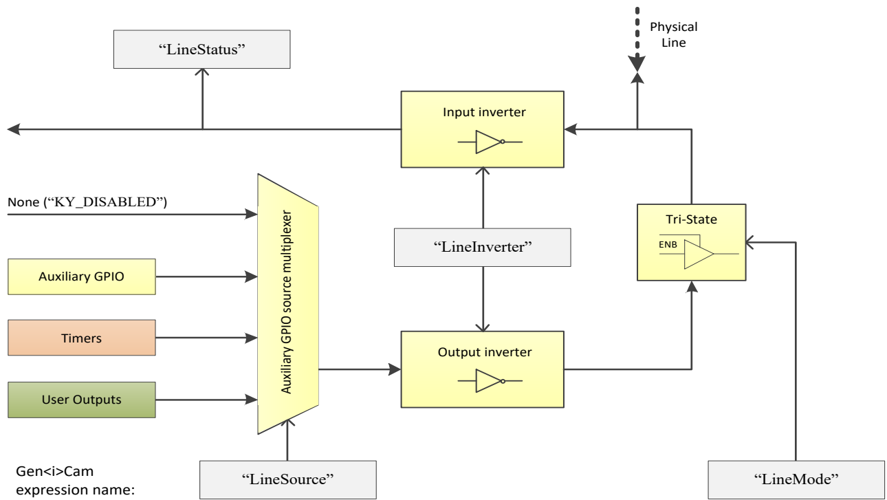
Figure 29 – Digital I/O Line structure
