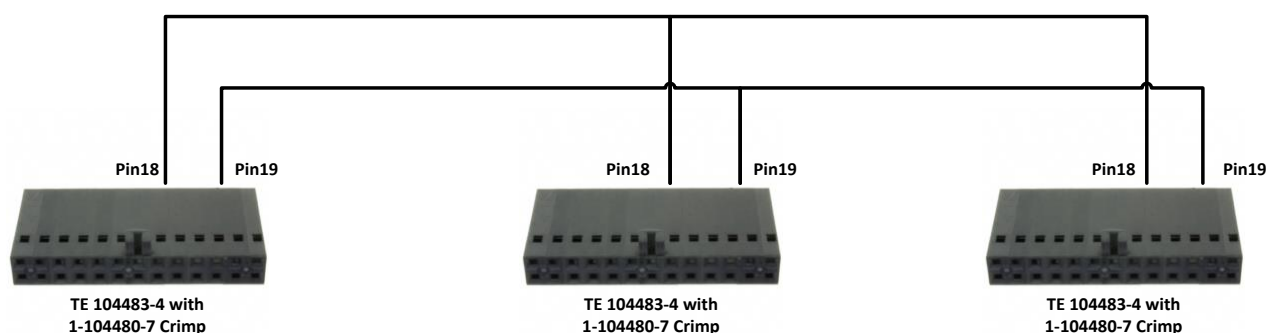
Figure 33 – Frame Grabber synchronization wiring
