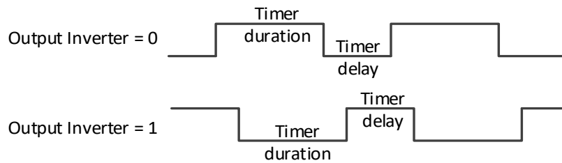
Figure 28 – Output inverters
