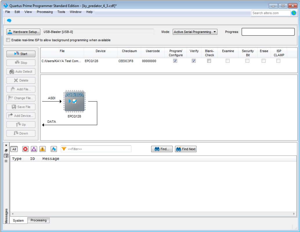
Figure 5 : Quartus – Programming Configuration
