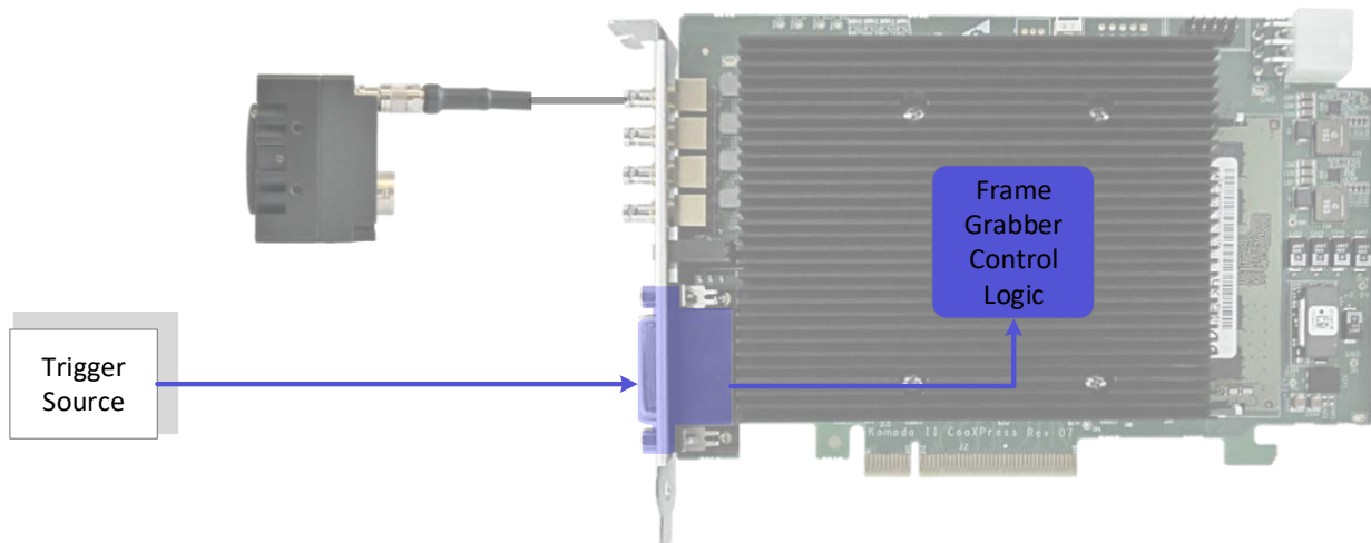
Figure 23 – Acquisition stream trigger source
