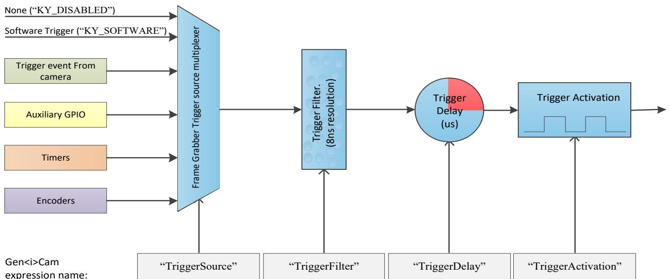
Figure 24 – Acquisition stream trigger structure
