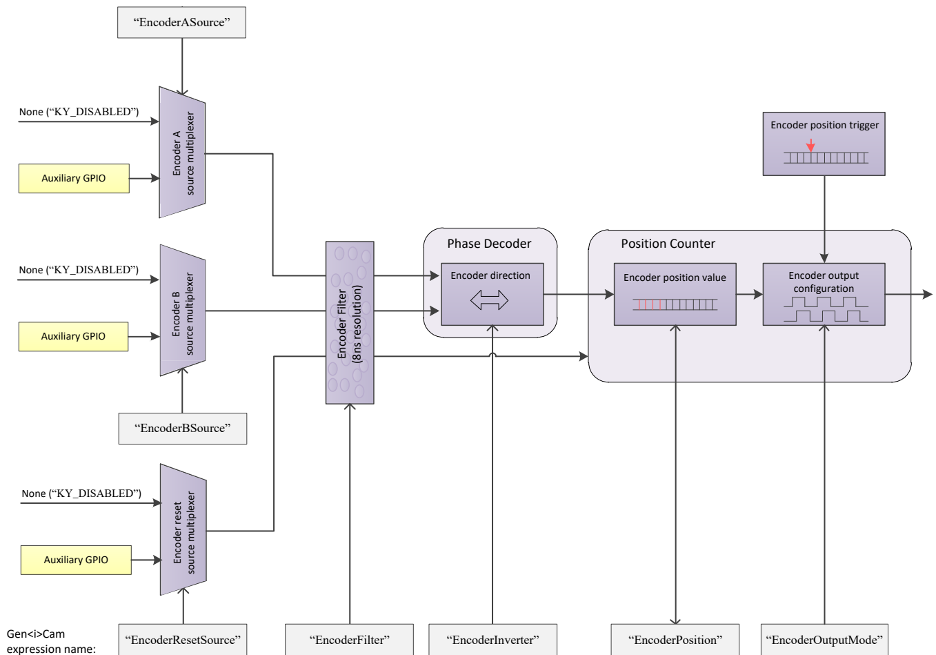
Figure 25 – Encoder triggers structure
