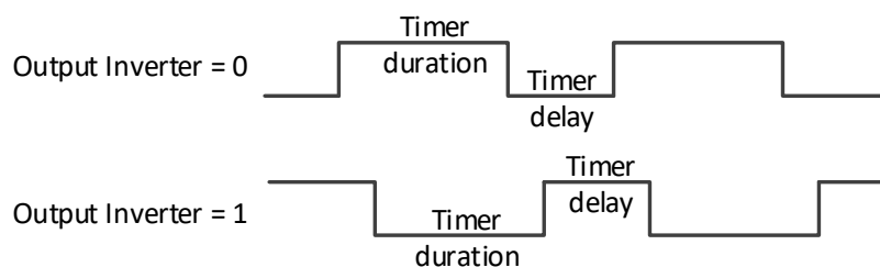
Figure 28 – Output inverters
