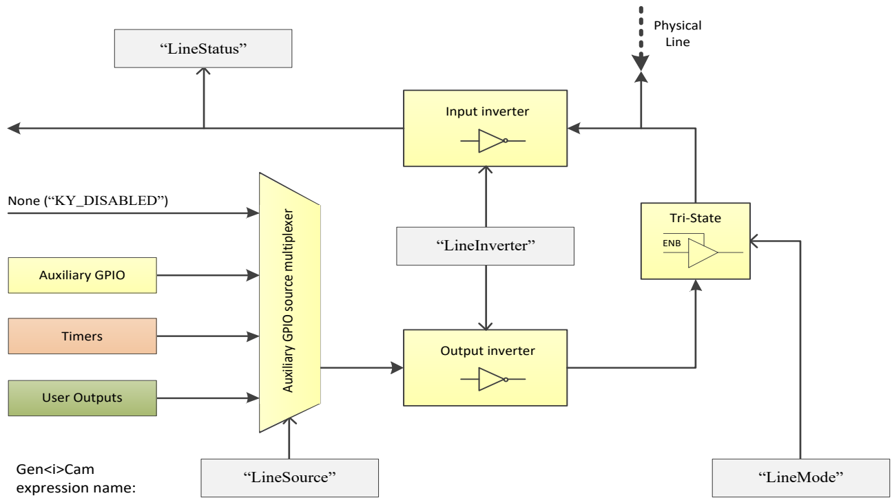
Figure 29 – Digital I/O Line structure
