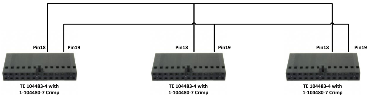
Figure 33 – Frame Grabber synchronization wiring
