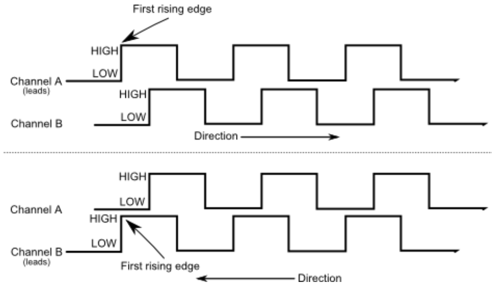
Figure 26 – Encoder channels
