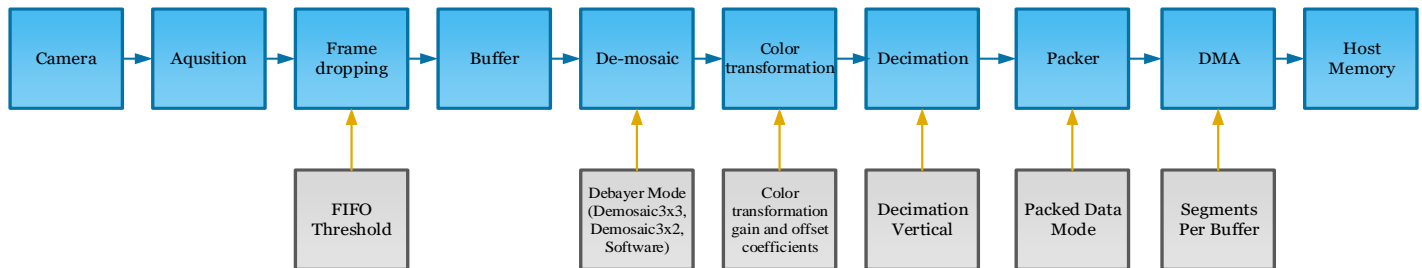
Figure 12 – Hardware based image processing pipeline
