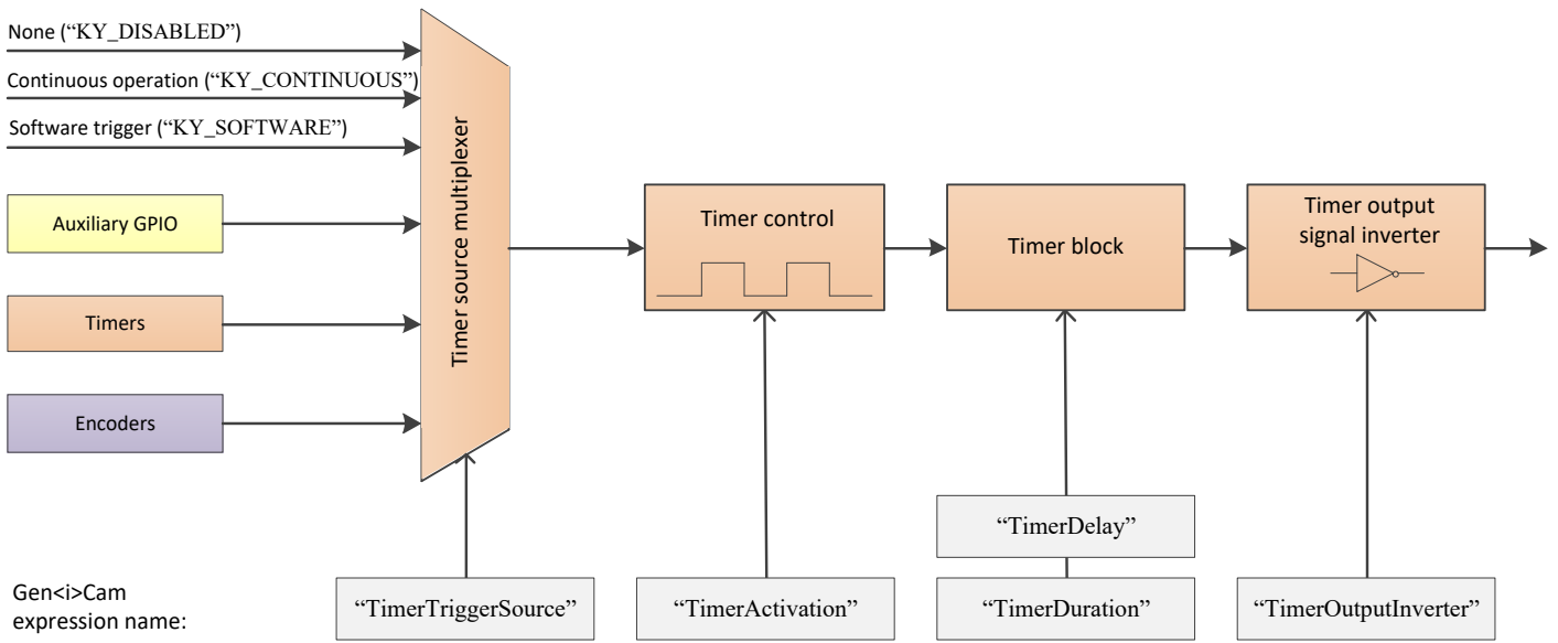
Figure 27 – Timer triggers structure
